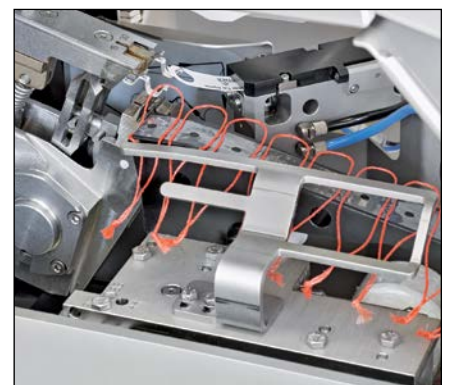
Label is securely attached to the product together with the clip and the loop.
